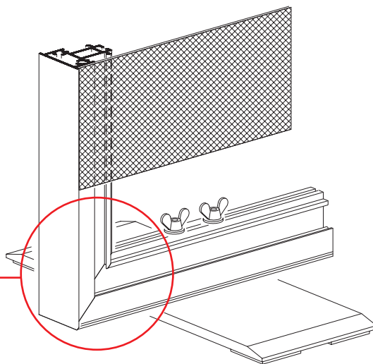
base plate M 1347 120 x 320 mm Fussplatte M 1347120 x 320 mm
